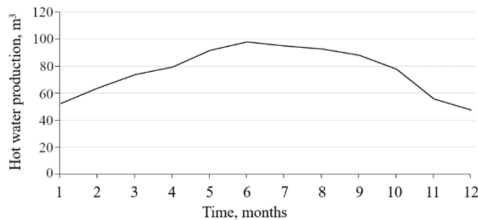
Fig. 5. Volumetric heating output of a solar water heater when heating 1 \text{ m}^3 water to a temperature of 44^\circ\text{C} by months
