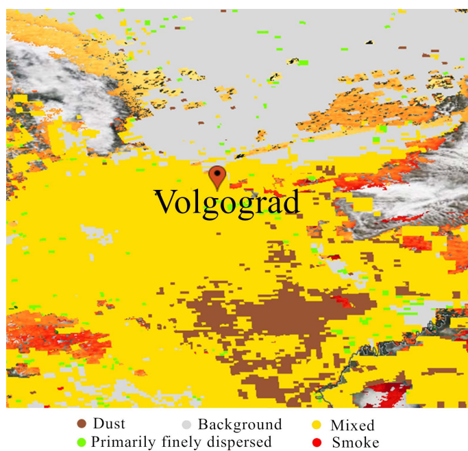
Fig. 7. Satellite data of MODIS (flight time 10:28 UTC) and VIIRS (flight time 10:02 UTC) for 30 May 2024: AOD distribution from the MAIAC algorithm (a), aerosol type determination from the VIIRS Deep Blue algorithm (b)
